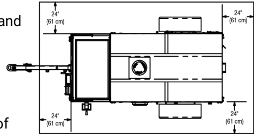
Figure 18 - Top-View Clearances
