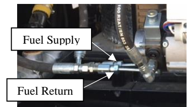
Figure 25 - Riello Burner Side (Fuel Lines)
