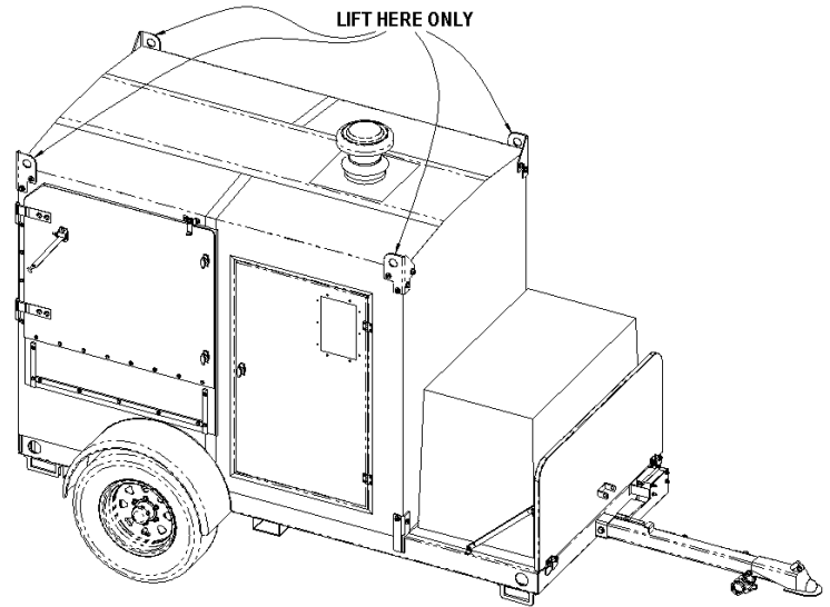
Figure 14 - Lifting Points
