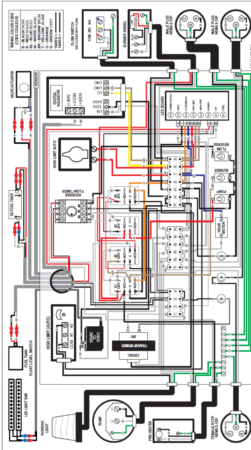
Figure 53 - 200 GTS C/W Optional Flow Reverser Electrical Schematic
