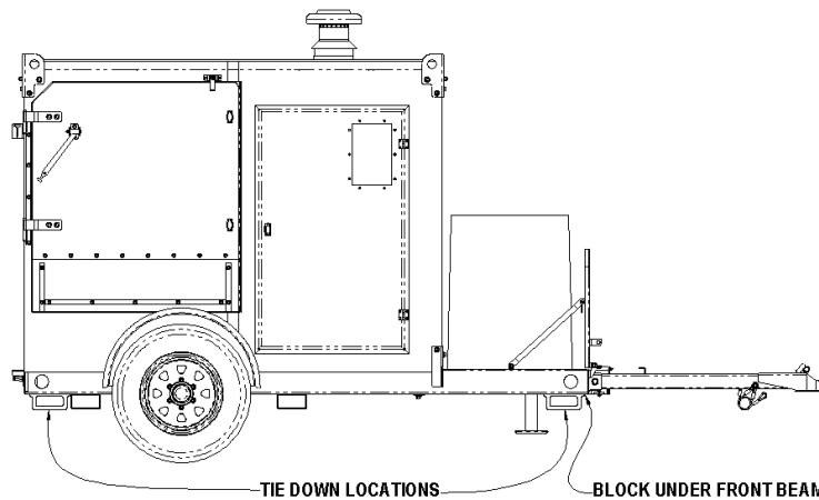
Figure 17 - Tie-Down Points
