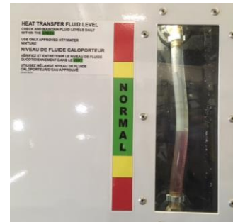
Figure 38 - HTF Level Indicator
