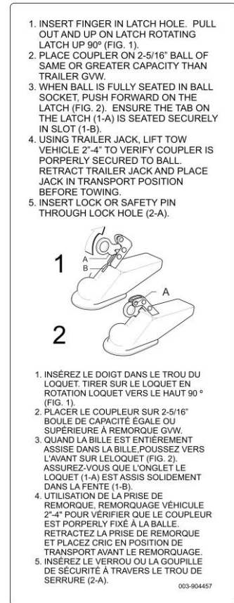
Figure 2 - Trailer Coupler
